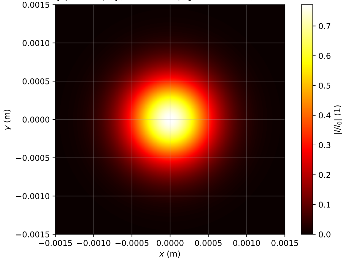
Intensity profile I(x, y, z = 1.592m)/I_0 , Pin=0.3Pcr, artificial time
